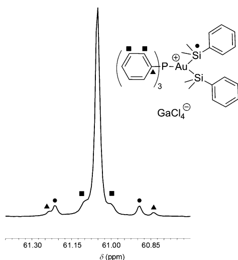
Figure 1. Long-acquisition ^{31}\text{P}\{^1\text{H}\} spectrum of complex 1a that shows the ^{13}\text{C} (▲ and ■) and ^{29}\text{Si} (●) satellites.
